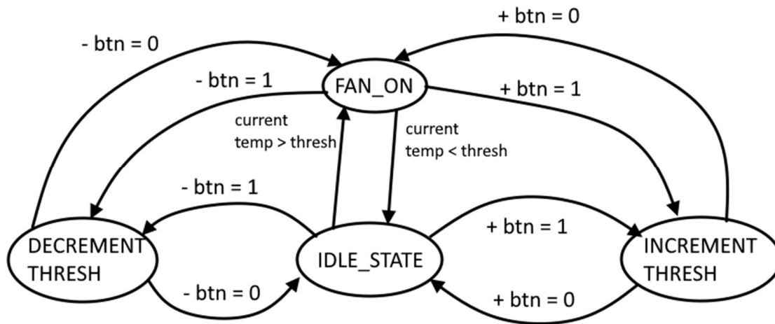
Figure 1: Diagram for Finite State Machine
